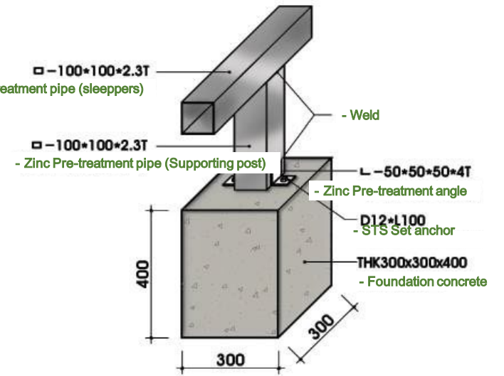
▲ The lower details
