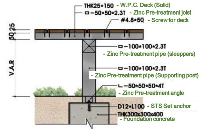
▲ Deck install details
