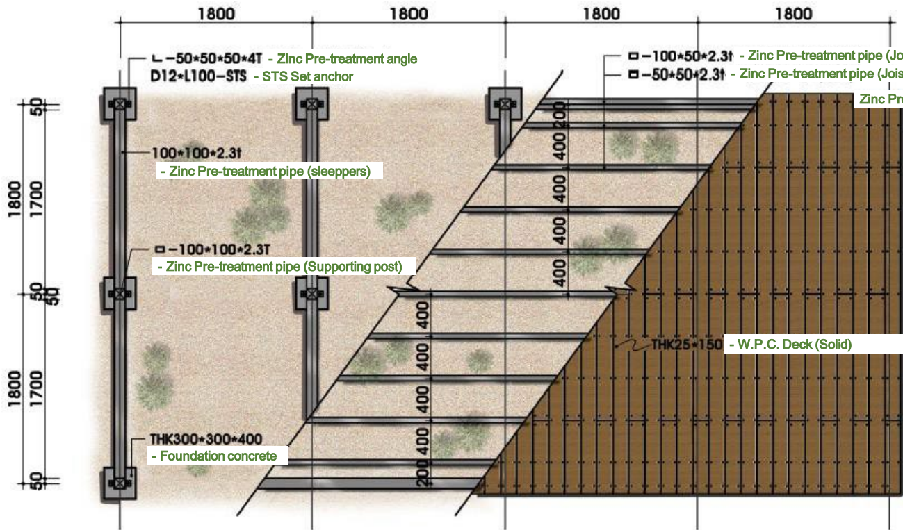
▲ Sleepers details
